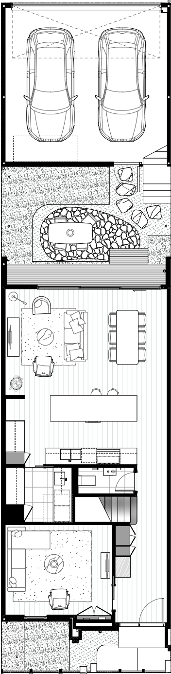
Ground Floor
