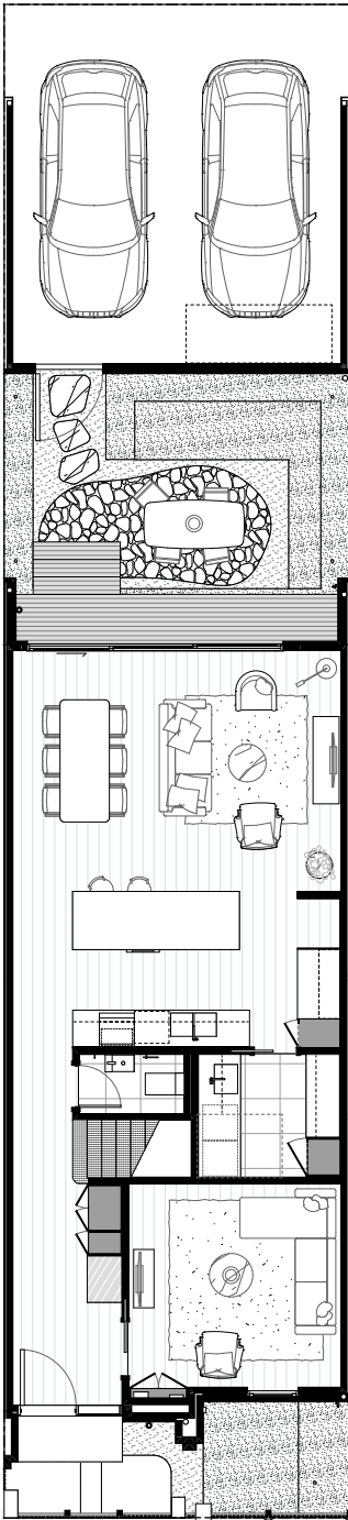
Ground Floor
