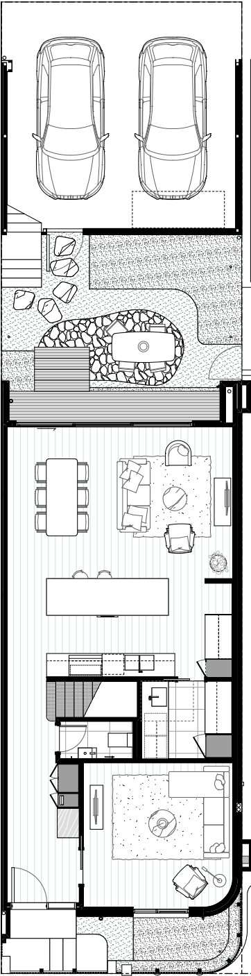
Ground Floor
